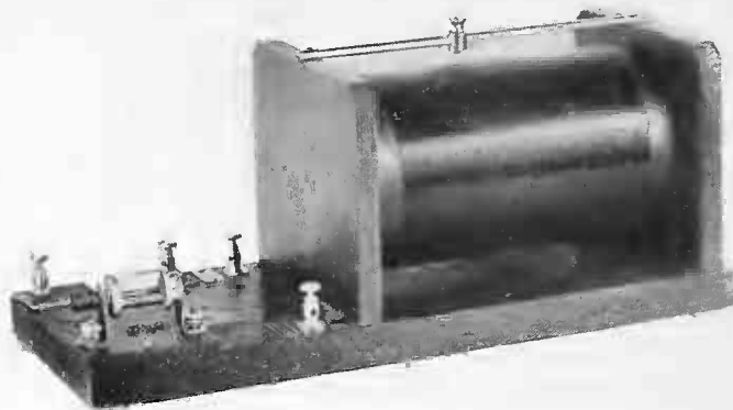
TYPE "ML" RECEIVER SET
