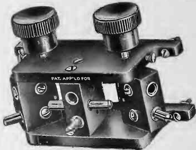
The New Amco Adjustable Triple Coil Mounting
